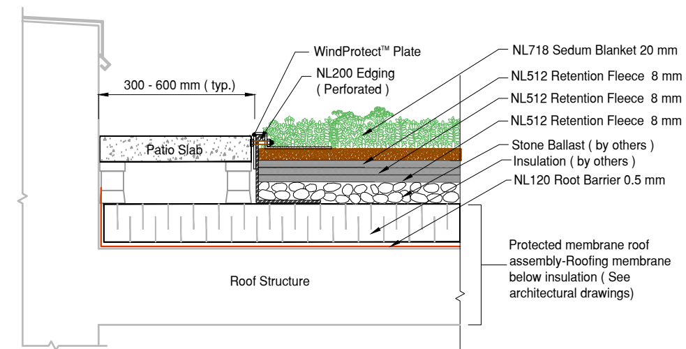
2 DET LiteN'Less Classic III 718 with Edge Paver Edge Detail Protected Membrane Roof
