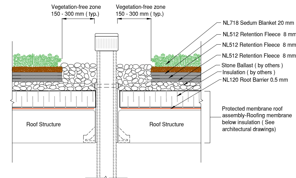
4 DET LiteN'Less Classic III 718 with Edge Penetration Detail Protected Membrane Roof
