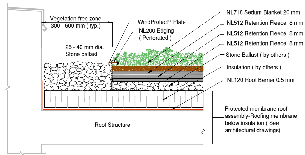
1 DET LiteN'Less Classic III 718 with Edge Stone Edge Detail Protected Membrane Roof
