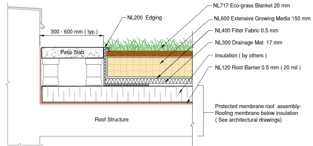
2 DET Eco-Grass Paver Edge Detail Protected Membrane Roof
