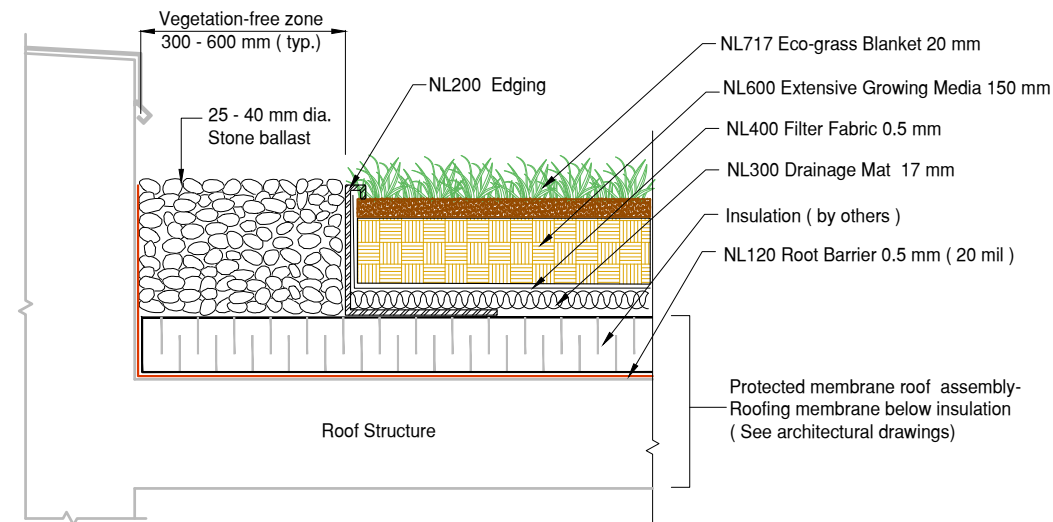
1 DET Eco-Grass Stone Edge Detail Protected Membrane Roof
