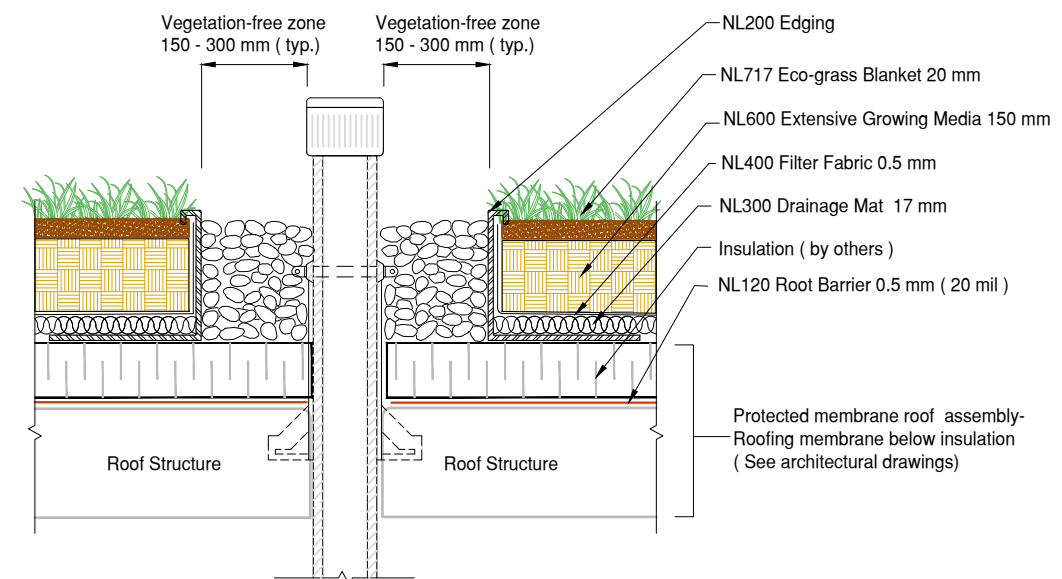
4 DET Eco-Grass Penetration Detail Protected Membrane Roof
