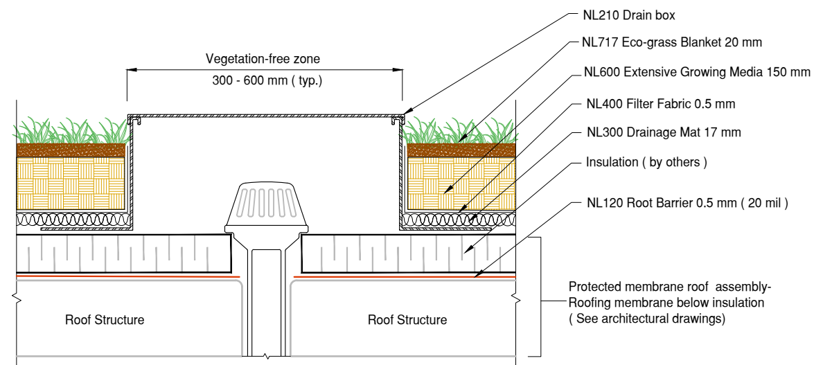
3 DET Eco-Grass Drain Detail Protected Membrane Roof
