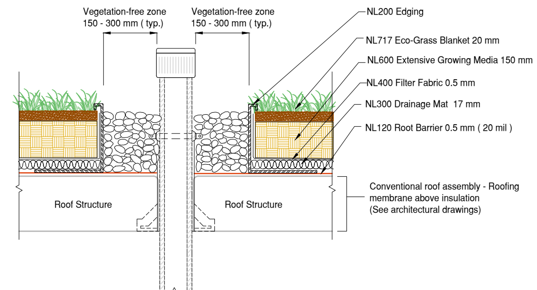
4 Eco-Grass Penetration Detail DET Conventional Roofing Assembly
