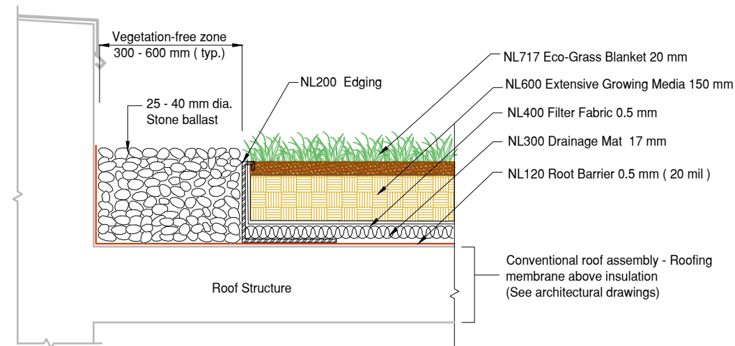
1 Eco-Grass Stone Edge Detail DET Conventional Roofing Assembly
