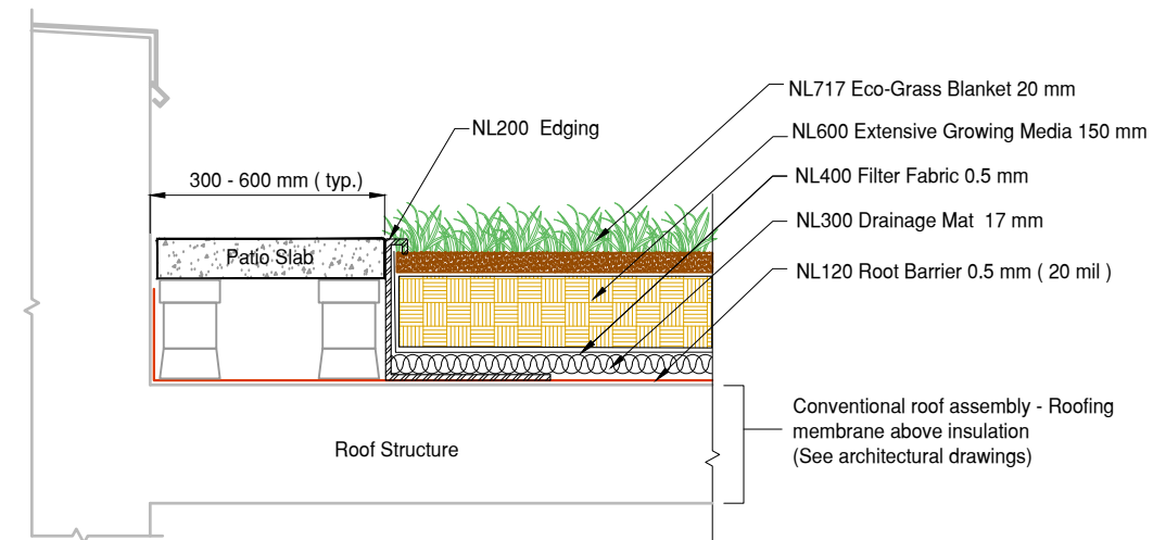
2 Eco-Grass Paver Edge Detail DET Conventional Roofing Assembly
