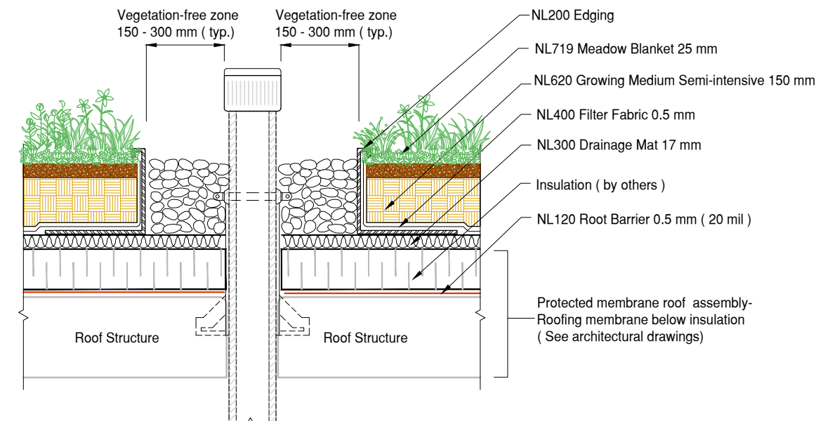
4 Alpine Meadow Penetration Detail DET Protected Membrane Roof
