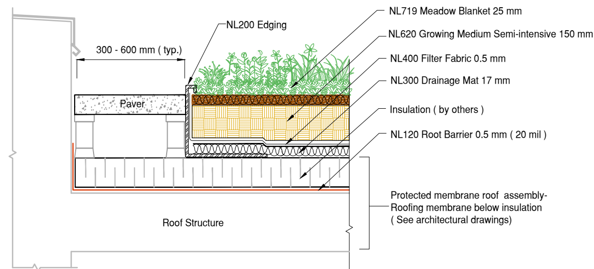
2 Alpine Meadow Paver Edge Detail DET Protected Membrane Roof
