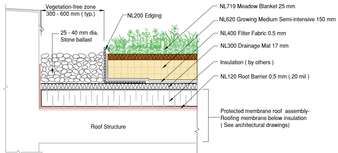
1 Alpine Meadow Stone Edge Detail DET Protected Membrane Roof
