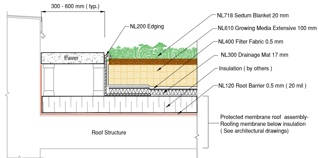
2 DET TerraEXT Standard Paver Edge Detail Protected Membrane Roof
