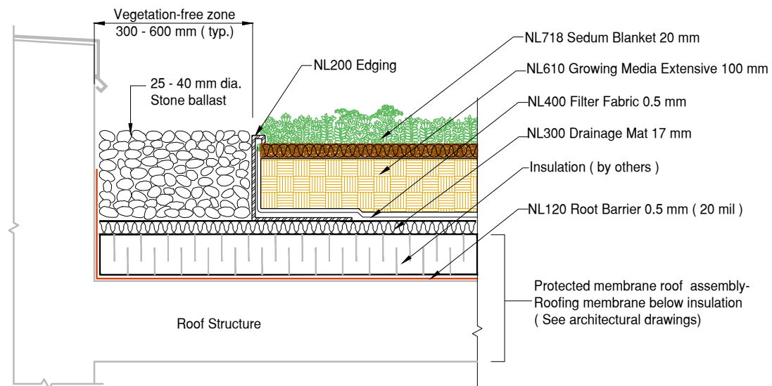
1 DET TerraEXT Standard Stone Edge Detail Protected Membrane Roof
