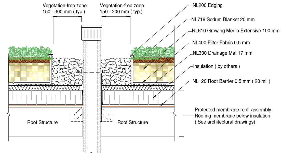
4 DET TerraEXT Standard Penetration Detail Protected Membrane Roof
