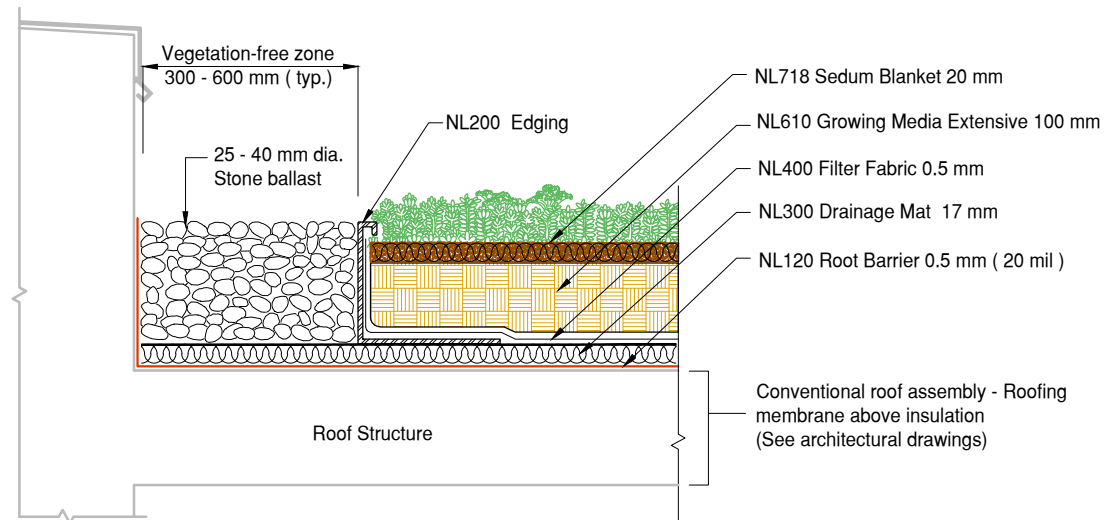
1 TerraEXT Standard Stone Edge Detail DET Conventional Roofing Assembly
