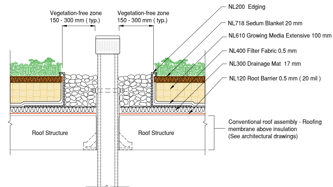
4 Terra EXT Standard Penetration Detail DET Conventional Roofing Assembly
