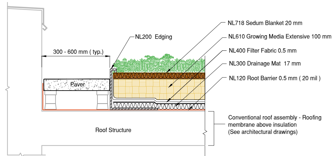
2 TerraEXT Standard Paver Edge Detail DET Conventional Roofing Assembly
