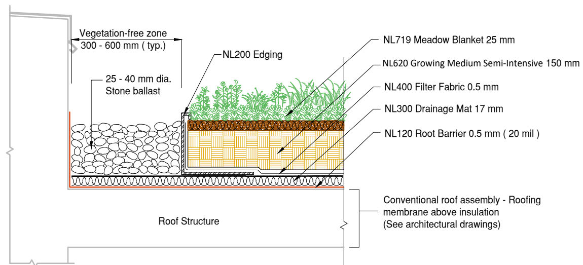
1 DET Alpine Meadow Stone Edge Detail Conventional Roofing Assembly
