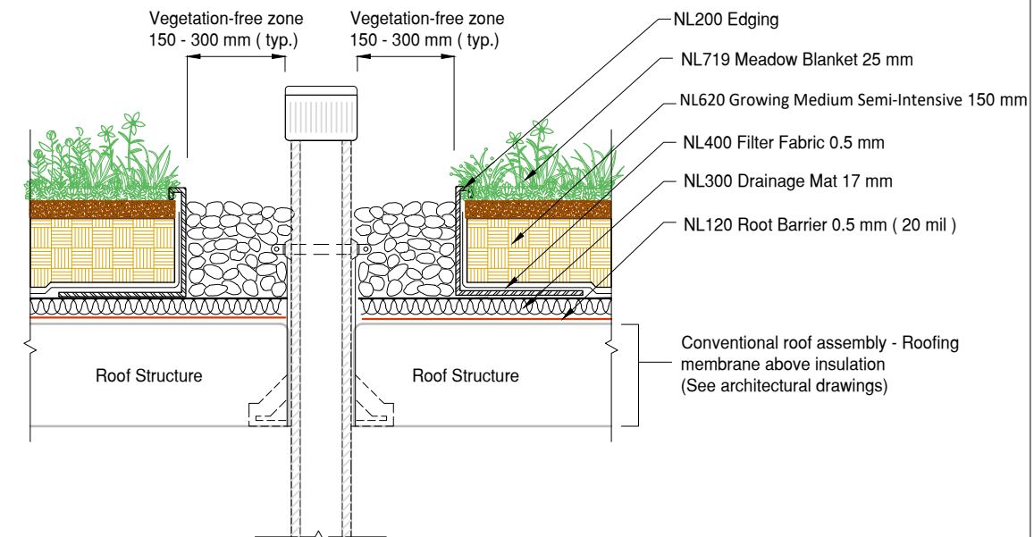
4 DET Alpine Meadow Penetration Detail Conventional Roofing Assembly
