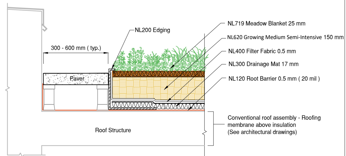
2 DET Alpine Meadow Paver Edge Detail Conventional Roofing Assembly
