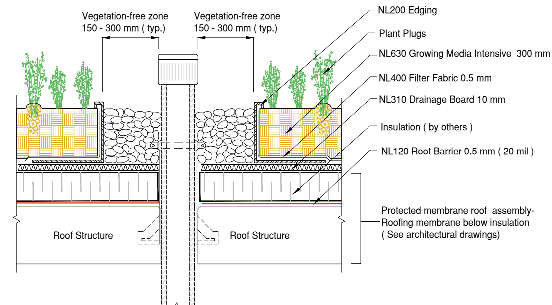
4 Flora Garden Penetration Detail
