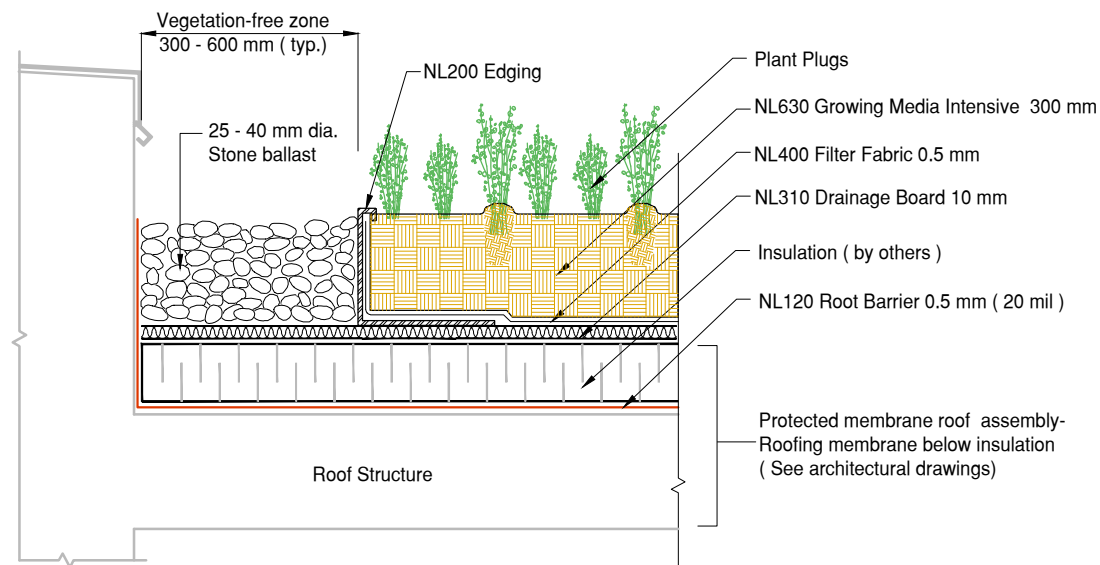
1 Flora Garden Stone Edge Detail
