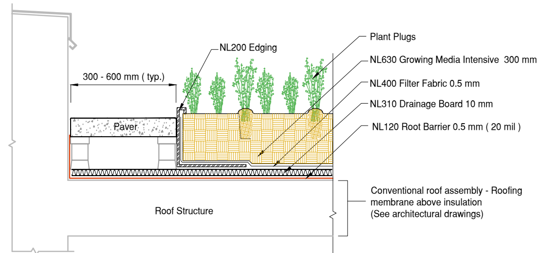
2 DET Flora Garden Paver Edge Detail Conventional Roofing Assembly
