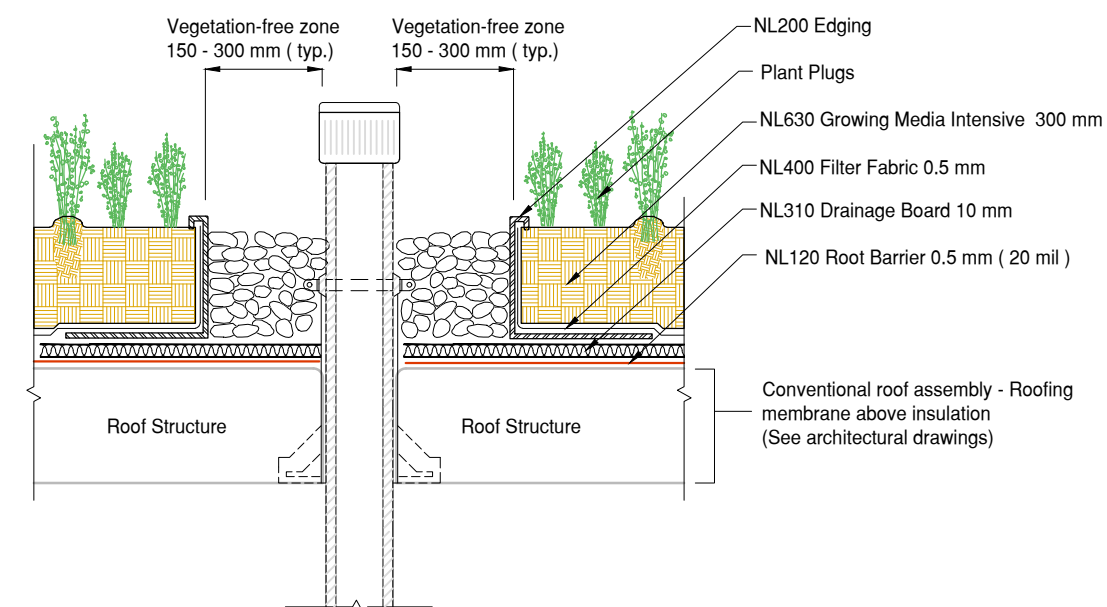
4 DET Flora Garden Penetration Detail Conventional Roofing Assembly
