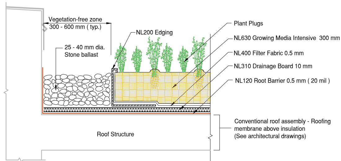
1 DET Flora Garden Stone Edge Detail Conventional Roofing Assembly
