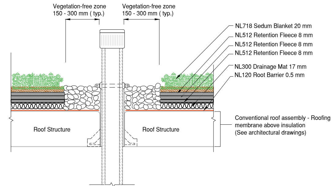
4 LiteN'Less Classic III 718 w/ Edge Penetration Detail DET Conventional Roofing Assembly
