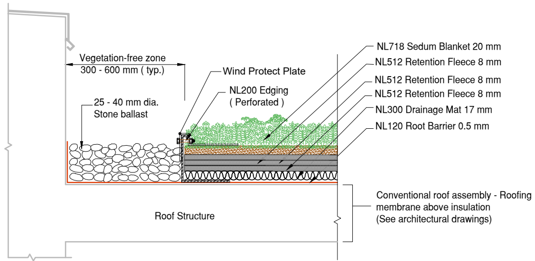
1 LiteN'Less Classic III 718 w/ Edge Stone Edge Detail DET Conventional Roofing Assembly
