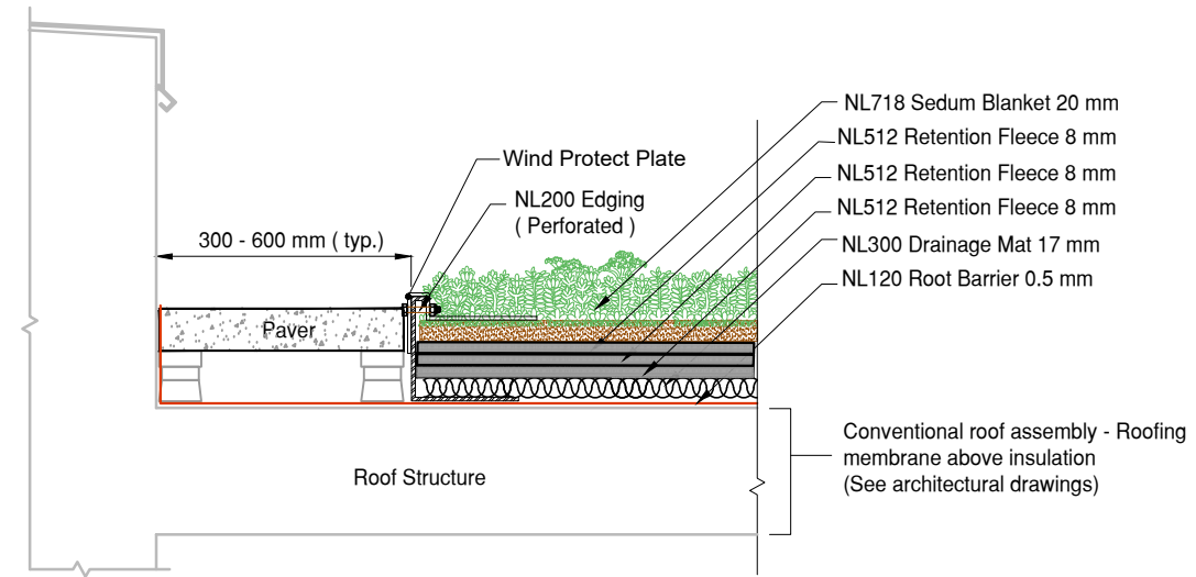
2 LiteN'Less Classic III 718 w/ Edge Paver Edge Detail DET Conventional Roofing Assembly
