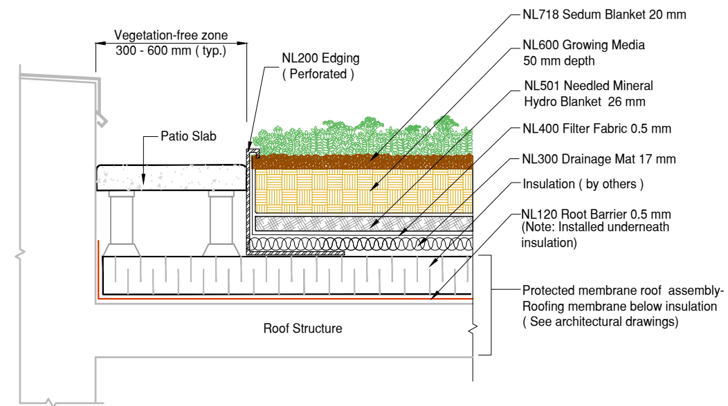
2 StormCap II System with Edge Paver Edge Detail DET Protected Membrane Roof
