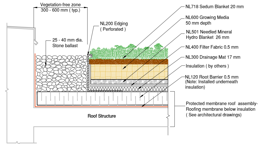
1 StormCap II System with Edge Stone Edge Detail DET Protected Membrane Roof
