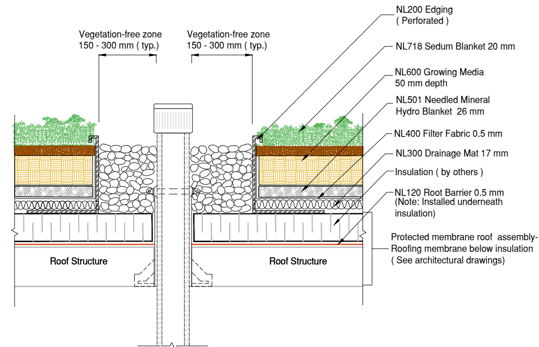
4 StormCap II System with Edge Penetration Detail DET Protected Membrane Roof
