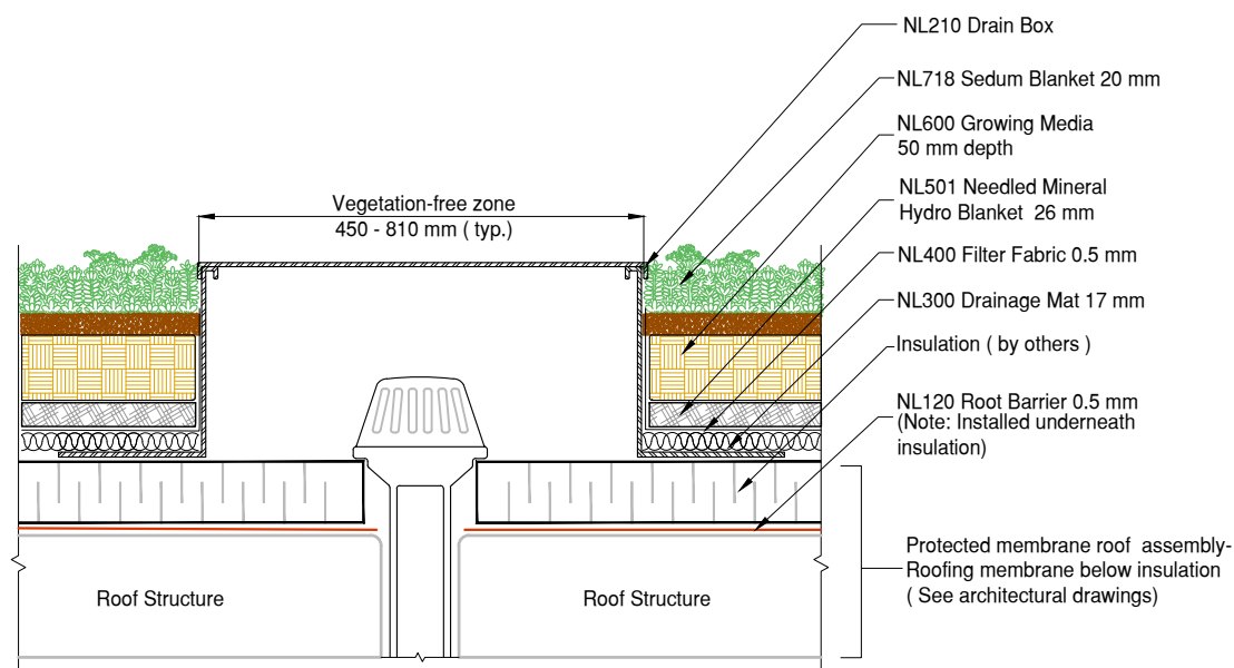
3 StormCap II System with Edge Drain Detail DET Protected Membrane Roof
