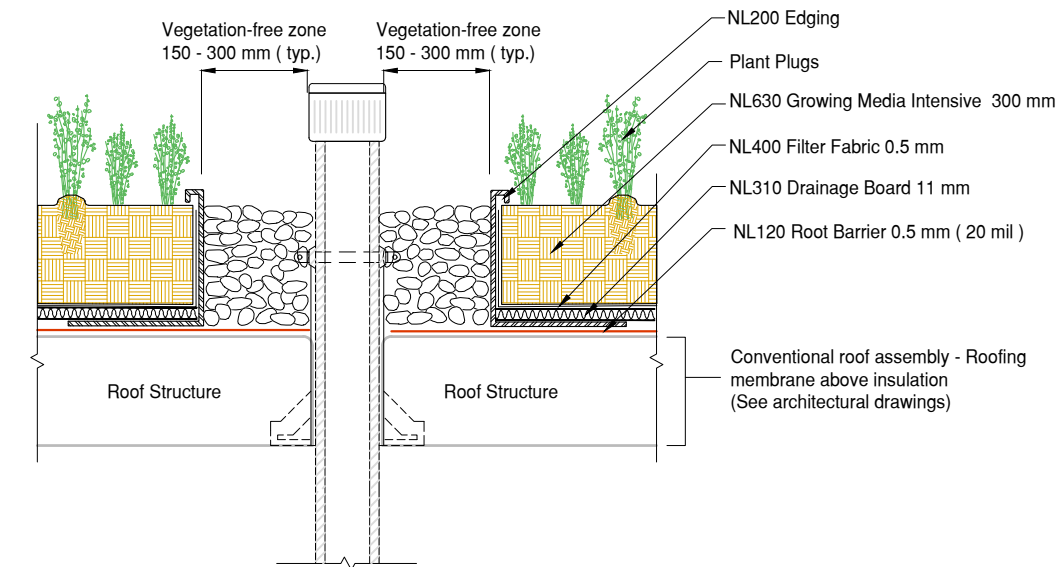
4 Flora Garden Penetration Detail DET Conventional Roofing Assembly
