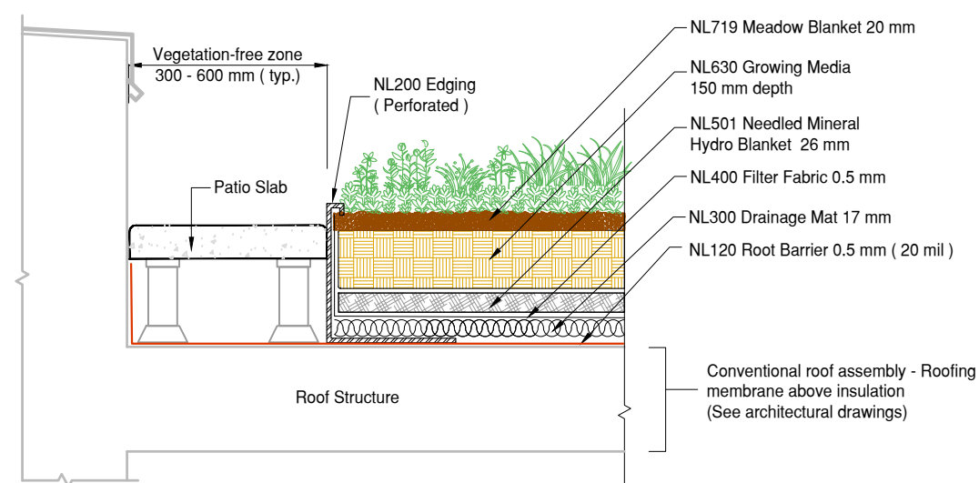
2 DET NL719 Alpine Meadow+ Paver Edge Detail Conventional Roofing Assembly
