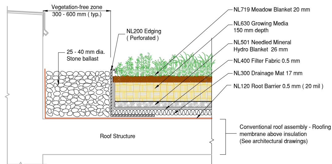
1 DET NL719 Alpine Meadow+ Stone Edge Detail Conventional Roofing Assembly
