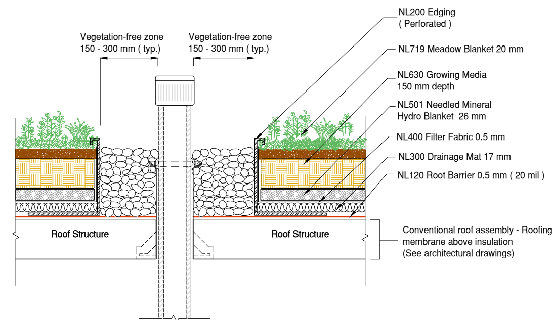
4 DET NL719 Alpine Meadow+ Penetration Detail Conventional Roofing Assembly
