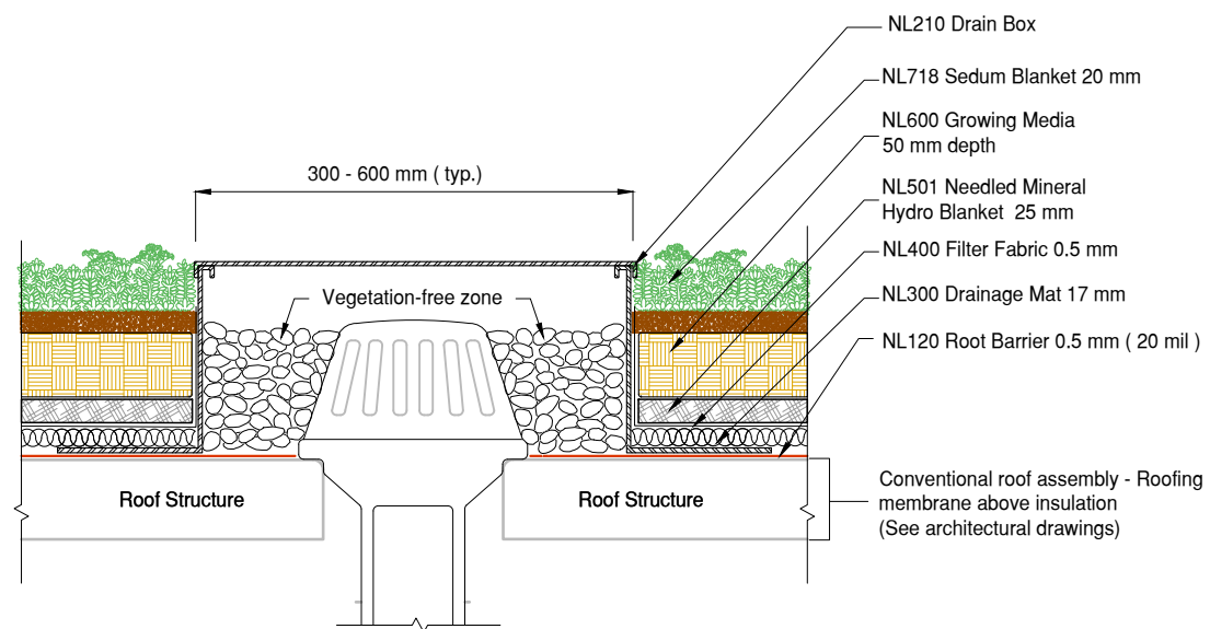
3 StormCap II System with Edge Drain Detail DET Conventional Roofing Assembly
